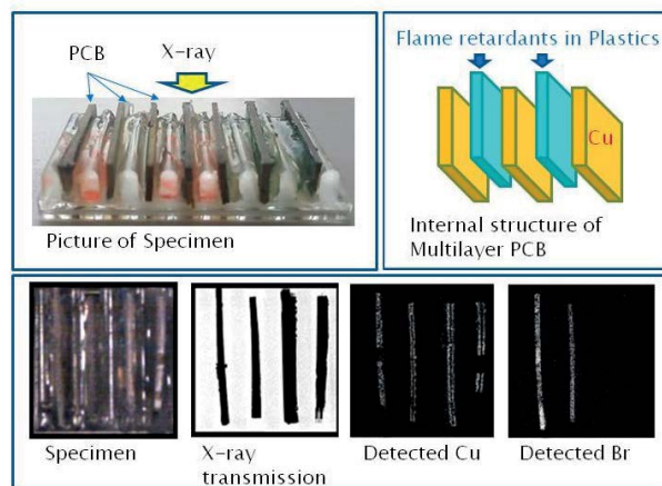
Figure 3: Specimen and the photo image by XGT.
