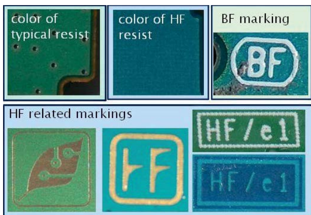
Figure 2: Examples of HF related markings provided by manufacturers RoHS1.
