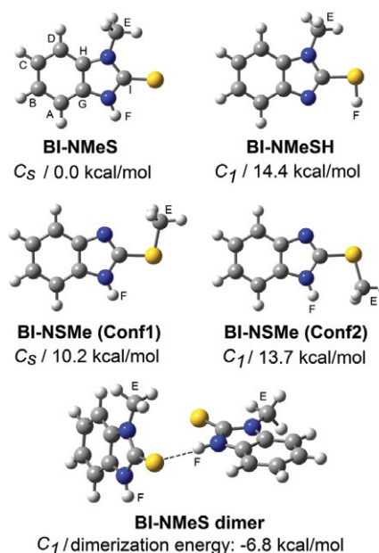
Figure 1: The geometrical structure, symmetry, and energetic stability of the investigated BI derivatives.
