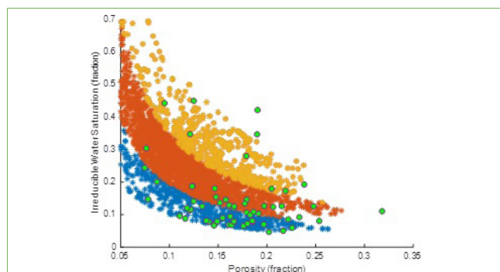
Figure 5: Rock type classification by BVW method and comparing its results with MICP data in field B.
