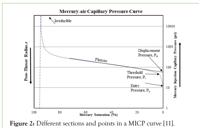
Figure 2: Different sections and points in a MICP curve [11].
