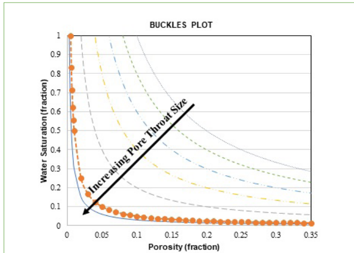
Figure 1: The bulk volume water plot .
