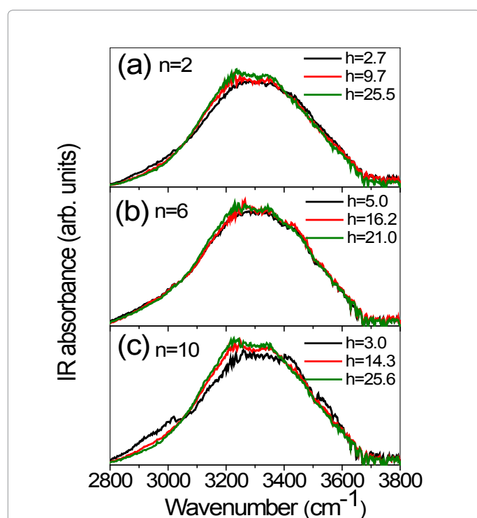
Figure 3: Examples of FTIR-ATR spectra of \gamma -CDEDTA1 n ( n = 2, 6, 10 ) hydrogels in the 2800 \div 3800 \text{ cm}^{-1} wavenumber region. (a) \gamma -CDEDTA12 hydrogel at h = 2.7 (black line), 9.7 (red line), 25.5 (green line); (b) \gamma -CDEDTA16 hydrogel at h = 5.0 (black line), 16.2 (red line), 21.0 (green line); (c) \gamma -CDEDTA110 hydrogel at h = 3.0 (black line), 14.3 (red line), 25.6 (green line).
