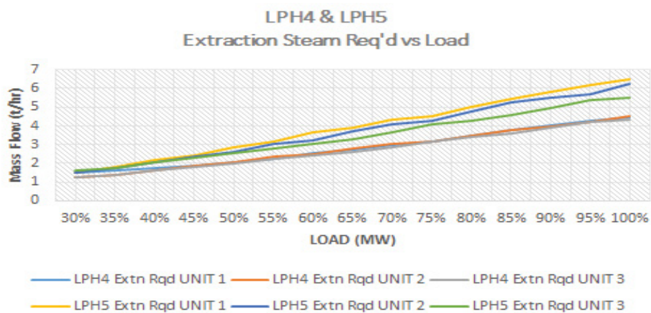
Figure 18: LPH4 and LPH5 extraction steam flow required.
