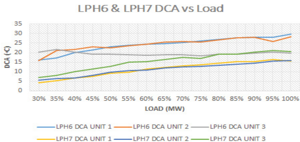
Figure 11: LPH6 and LPH7 DCA vs. load trend.
