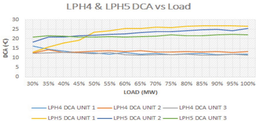
Figure 10: LPH4 and LPH5 DCA vs. load trend.
