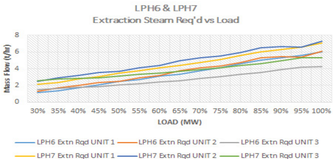
Figure 19: LPH6 and LPH7 extraction steam flow required.
