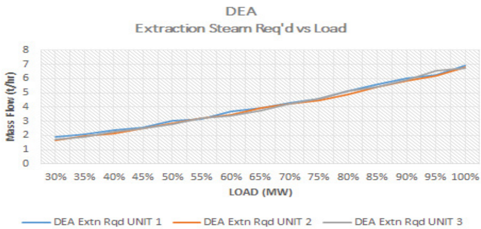
Figure 17: DEA extraction steam flow required.
