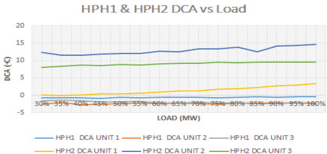
Figure 9: HPH1 and HPH2 DCA vs. load trend.
