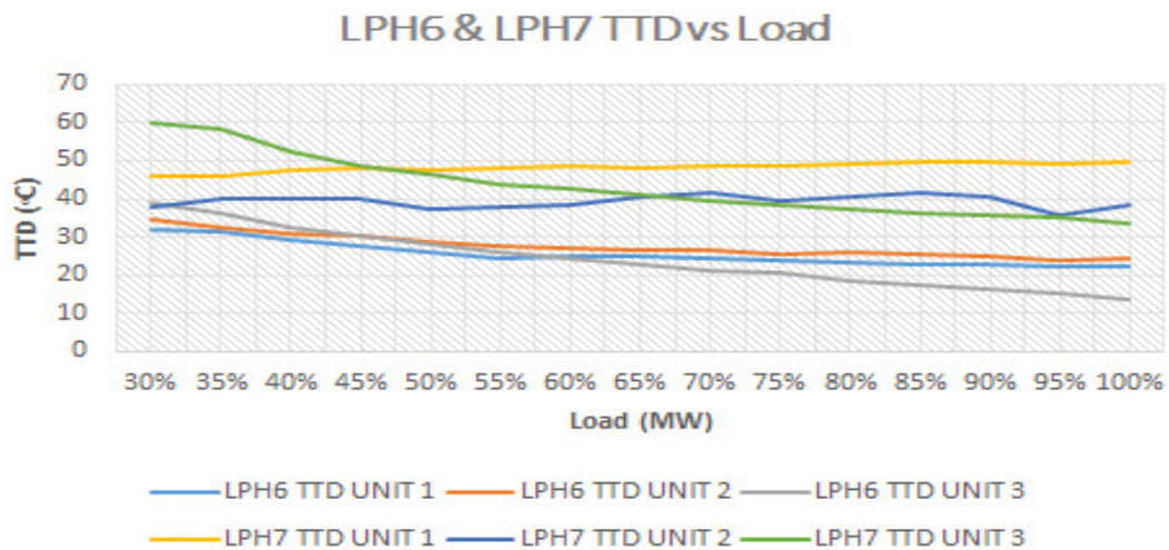
Figure 8: LPH6 and LPH7 TTD vs. load trend.
