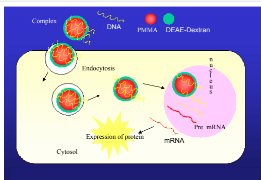
Figure 12: Schematic drawing of putative pathways for the delivery of foreign DNA in complex with DEAE-dextran-MMA graft copolymer.
