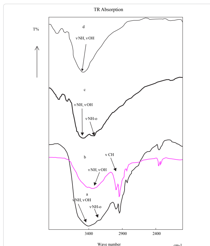
Figure 11: Infra-Red absorption spectra: a, DDMC/DNA complex; b, DDMC; c, DEAE-dextran/DNA complex; d, DEAE-dextran.
