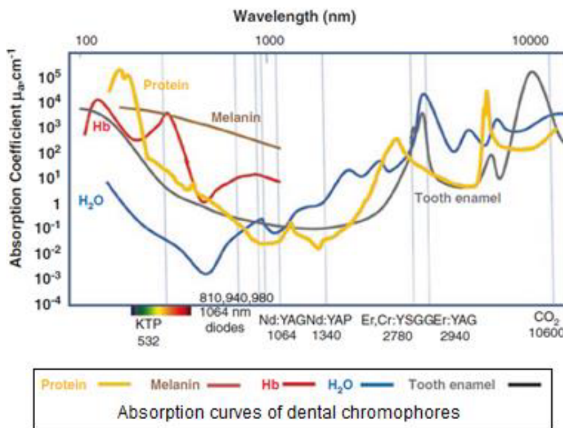
Figure 1: Absorption coefficient values of predominant chromophores (haemoglobin, melanin, apatite crystalline solids and water) relative to common laser wavelengths used in dentistry.
