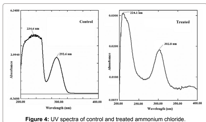
Figure 4: UV spectra of control and treated ammonium chloride.
