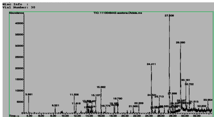
Figure 1: GCMS analysis of seagrass extract of H. ovalis .
