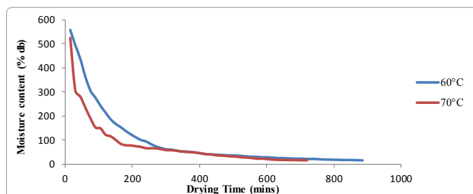
Figure 2: Drying curves of banana peel at different temperature.
