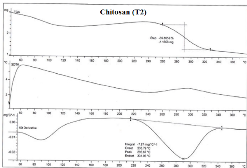
Figure 7b: TGA-DTG thermogram of chitosan (T2).
