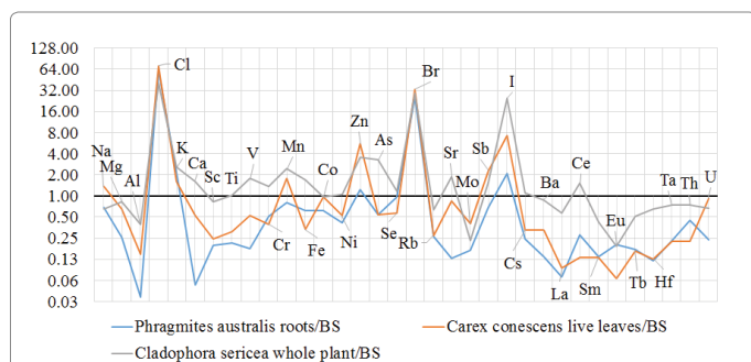
Figure 5: The elemental content of Phragmites australis , Carex conescens and Cladophora sericea normalized against bottom sediments.
