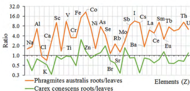
Figure 3: Average differences between leaves/roots ratios for Phragmites australis and Carex conescens .
