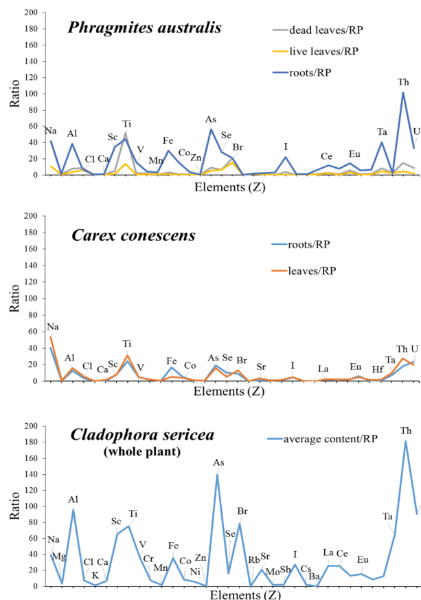
Figure 4: Studied plant/Reference plant ratios for different parts of Phragmites australis , Carex conescens and Cladophora sericea .
