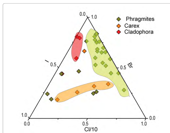
Figure 6: Ternary diagram for concentrations of Cl (Cl/10), Br and I for Phragmites australis , Carex conescens and Cladophora sericea normalized against content of these elements in sediments (BS). With some exceptions ( Phragmites samples), all other points form three distinct clusters corresponding to each type of plant.
