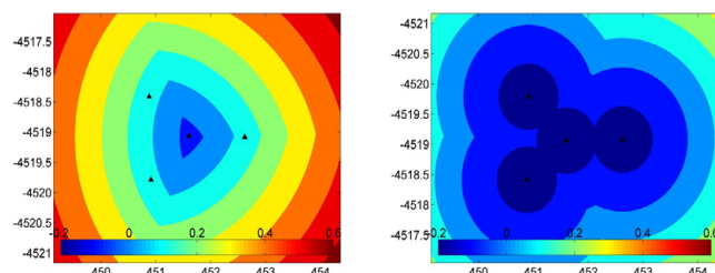
Figure 3: Sensitivity to location (left) and detection (right) power of a test network, which seismic stations are represented by black triangles) for earthquakes located at 2 km b.s.l. The color represents the value of the minimum magnitude needed for an earthquake in that position to be located/detected system by the network. Latitude and longitude are expressed in the UTM coordinate system (km).
