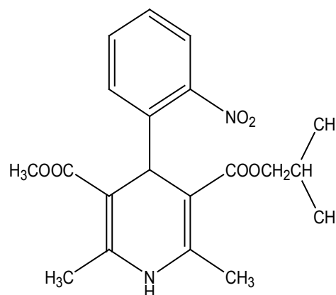
Figure 1: The chemical structure of Nisoldipine.
