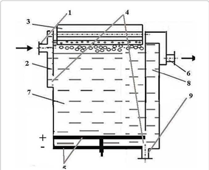
Figure 2: Electroflotator of continuous action for the juice concentration.
