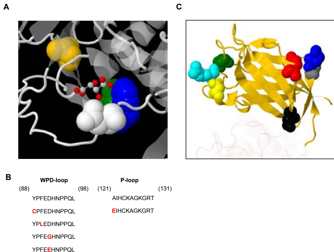
Figure 3: Mutations of tumor suppressor PTEN in HNSCC. Crystal structure of PTEN protein is represented as ribbon diagrams. A. The functional active pocket of the phosphatase domain is shown. The mutated residues in the WPD-loop are highlighted in green (Y88), blue (F90), and white (D92). The mutated residue A121 is in yellow. B. Sequence of the WPD-loop and P-loop depicting the mutated residues within the walls of the active pocket present in the PTEN phosphatase domain. Mutated amino acid residues are in red. C. Mutated residues Q245 (in blue) and R335 (in cyan) in the C2 domain are nonsense mutations. Y225, P246, and D252 are shown in red, gray, and black respectively. M205 (in green) is in the C \beta 1/2 loop; and D331G (in yellow) is in the C2 \alpha loop.
