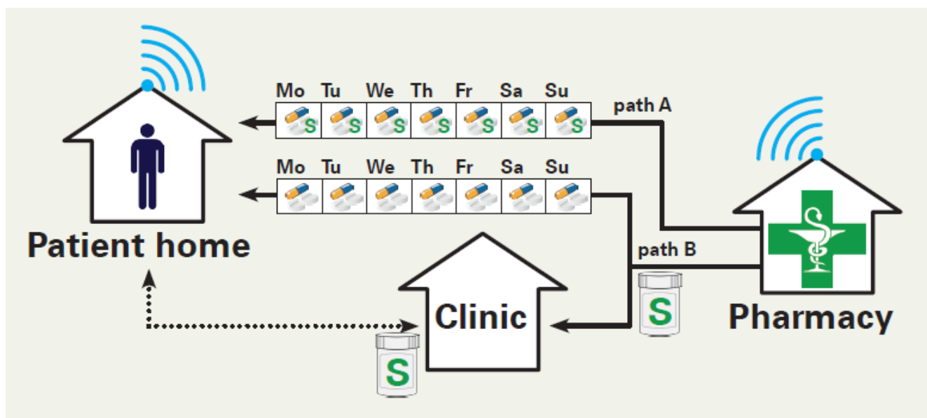
Figure 3: Novel medication supply model where the community pharmacy provides unit-of-dose pouches (medication roll Mo-Su) with the solid oral medications directly to patient home, including opioid (path A). Depending on the regulations in force, patients with opioid agonist therapy must obtain the opioid (S) at the outpatient addiction clinic in regular intervals, in Switzerland at least once weekly (dotted line). For these patients, the pharmacy delivers the opioid agonist directly to the clinic (path B). At the patient home, the pouches are loaded into a lockable, remote-controlled dispenser that can be programmed according to a patient's medication schedule. The dispenser records dates and times of medication retrievals and wirelessly transmits them to a server (blue waves).
