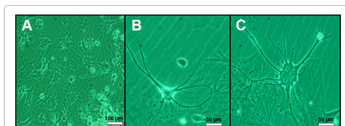
Figure 3: Phase-contrast microscopy of SC and DRG slices cultured in NVR-Gel 8 days after vitrification. (A) Neuronal and glia migration (B) A round DRG neuron which exhibits regenerated nerve fibers, euchromatic nucleus with a prominent nucleolus. (C) A multipolar SC nerve cell with regenerated nerve fibers.
