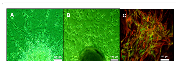
Figure 4: Regeneration of nerve fibers and migration of neuronal and glial cells from SC and DRG slices of rat fetuses cultured for 3 days (A&B) and 15 days (C) in NVR gel after vitrification. (A&B) Phase-contrast microscopy, (C) immunofluorescent double staining of migrated cells. Glial cells are marked in red (anti S-100 antibodies) and neurons in green (anti neurofilament antibodies).
