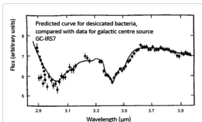
Figure 1a: The first prediction of the bacterial model of interstellar dust compared with the observations of the Galactic Centre infrared source GC-IRS7. The agreement implied that 30 percent of the carbon in interstellar space is tied up in the form of dust that cannot be spectroscopically distinguished from freeze dried bacteria.
