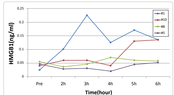
Figure 1: Increase in HMGB1 in plasma of LPS-injected monkeys.
