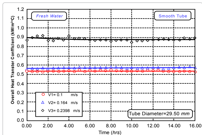
Figure 8: U versus time for time, with fresh water For various used flow speeds & D = 29.50 mm.
