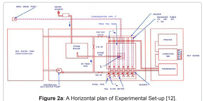
Figure 2a: A Horizontal plan of Experimental Set-up [12].
