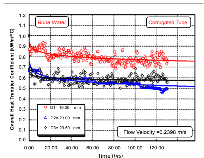
Figure 10: Variation of the overall heat transfer coefficient (U), with time for corrugated tube with Brine water, on different tube diameters, and flow velocity 0.2398 m/s.
