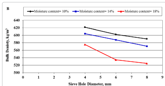
Figure 10: Effect of moisture content and sieve holes diameter on bulk density of corn crushed.
