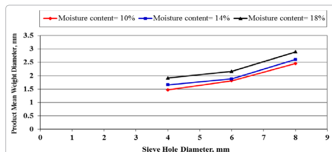
Figure 7: Effect of moisture content and sieve holes diameter on product mean weight diameter.
