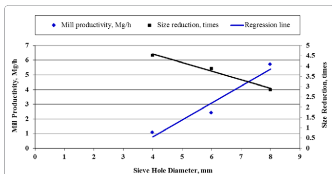
Figure 12: The relationship between the mill sieve hole diameter and both size reduction and mill productivity.
