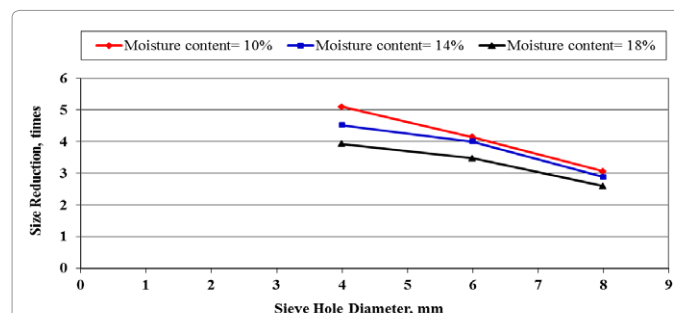
Figure 8: Effect of moisture content and sieve holes diameter on sizereduction.
