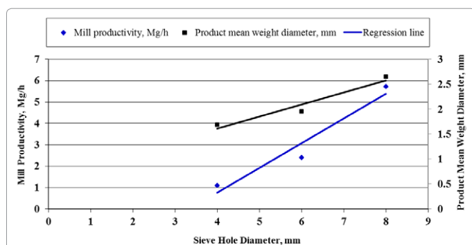
Figure 11: The relationship between the mill sieve hole diameter and both mill productivity and product mean weight diameter.
