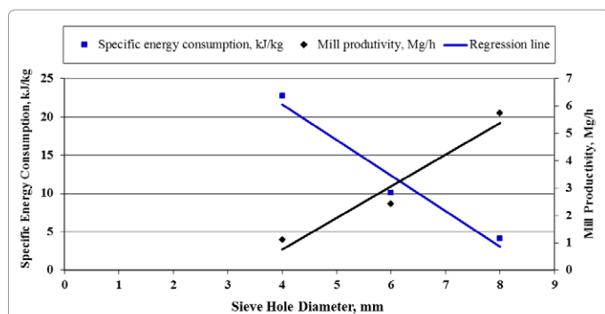
Figure 13: The relationship between the mill sieve hole diameter and both mill productivity and specific energy consumption of grinding.
