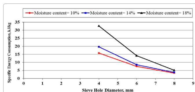
Figure 3: Effect of moisture content and sieve holes diameter on specific energy consumption of corn grinding.
