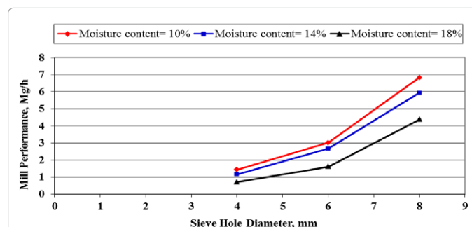
Figure 2: Effect of moisture content and sieve holes diameter on mill performance.
