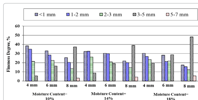
Figure 9: Effectof sieve hole diameter and cereal moisture contenton thefineness degree.
