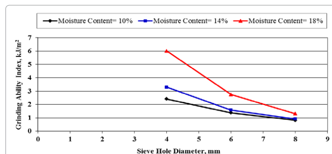
Figure 6: Effect of moisture content and sieve holes diameter on grinding ability index.
