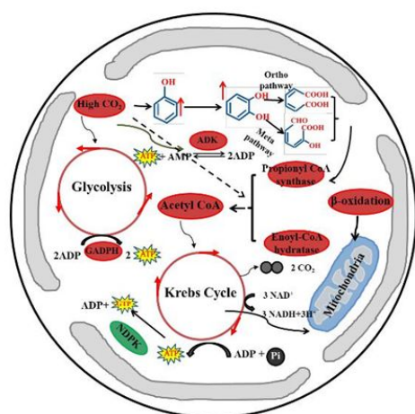
Figure 1: Ocean acidification up-regulated (red) and down-regulated (green) metabolic pathways in a calcifying microalga ( Emiliania huxleyi ) Jin et al. [9].
