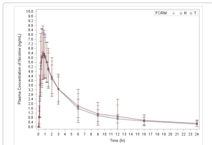
Figure 1: Mean graph (linear) for plasma concentration vs. time profile of nicotine after oral dose of nicotine 2 mg chewing gum (without baseline adjusted). Each point represents the mean+standard deviation. (n=43). O: (Reference) NICORETTE® Freshmint 2 mg Gum; O: (Test) Nicotine 2 mg Mint Flavored Chewing Gum.
