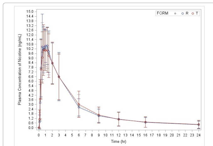
Figure 2: Mean graph (linear) for plasma concentration vs. time profile of nicotine after oral dose of nicotine 4 mg chewing gum (without baseline adjusted). Each point represents the mean+standard deviation. (n=37). O: (Reference) NICORETTE® Freshmint 4 mg Gum; O: (Test) Nicotine 4 mg Mint Flavored Chewing Gum.
