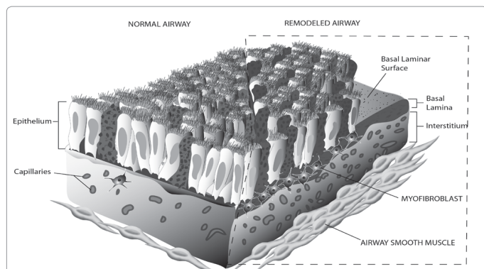
Figure 1: Airway Remodeling. The schematic above is split figure with normal airway represented on the left and a remodeled asthmatic airway on the right. The key features of the remodeled airway include mucous cell hyperplasia, thickening of the basement membrane with associated proliferation of myofibroblast, increased vascular density and increased smooth muscle hypertrophy. Together these changes predispose to airway hyper-responsiveness.
