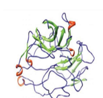
Figure 1: The final considered model from Modeller output (Visualisation by Chimerax).
