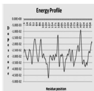
Figure 2: Analysis of the DOPE score profile of the model obtained from Modeller.
